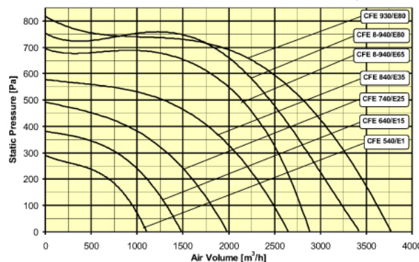
Type CFE .. single inlet, super flat Alternation Current: 230V/1N~, 50Hz
